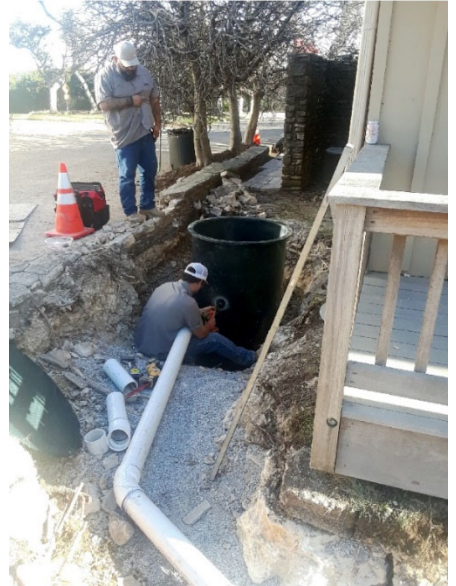
Trenching for main line and service line | Examples of equipment that may be used | Installing service line to grinder pump tank
